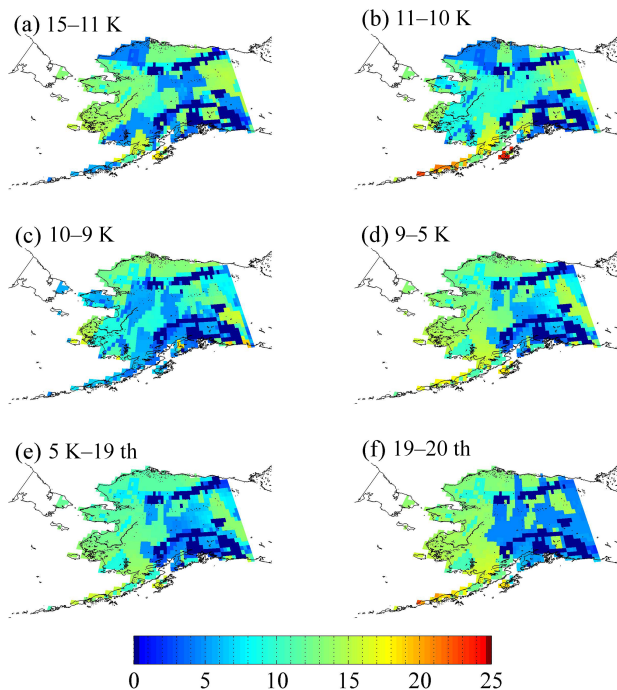
Figure 7. Average non-peatland (mineral) SOC density ( \text{kg C m}^{-2} ) during (a) 15–11 ka, (b) 11–10 ka, (c) 10–9 ka, (d) 9–5 ka, (e) 5 ka–1900 AD, and (f) 1900–2000 AD. The period of 9 k–19th in Fig. 2d is separated into 9–5 k and 5 k–19th.
