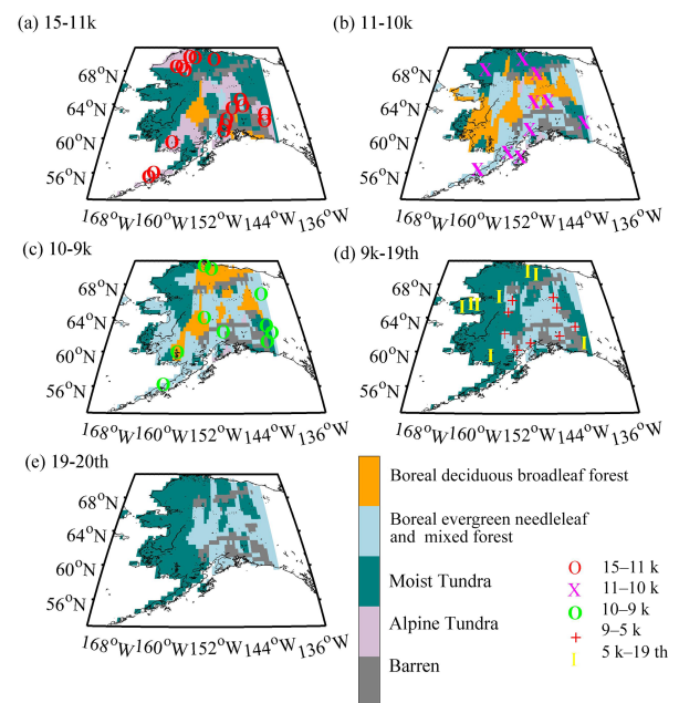
Figure 2. Alaskan vegetation distribution maps reconstructed from fossil pollen data during (a) 15–11 ka, (b) 11–10 ka, (c) 10–9 ka, (d) 9 ka–1900 AD, and (e) 1900–2000 AD (He et al., 2014). Symbols represent the basal age of peat samples ( n = 102 ) in Gorham et al. (2012). Each symbol indicates one to three peat samples in the map. Peat samples with basal age 9–5 k and 5 k–19th are shown in map (d) as there is no change in vegetation distribution during 9 k–19th. Barren refers to mountain range and large water body areas that can not be interpolated.
