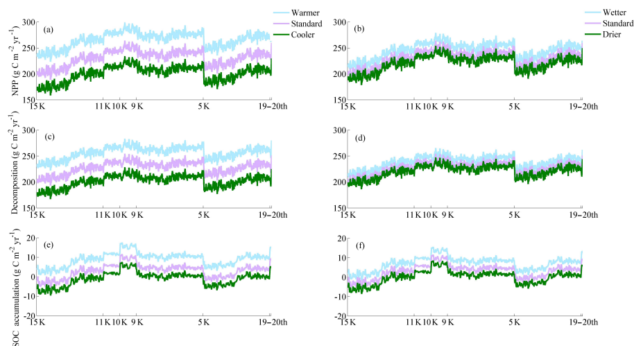
Figure 14. Temperature and precipitation effects on (a, b) annual NPP, (c, d) annual SOC decomposition rate (aerobic plus anaerobic), and (e, f) the annual SOC accumulation rate of Alaska. A 10-year moving average was applied.
