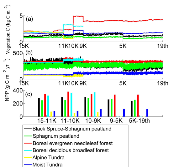
Figure 5. Simulated (a) mean vegetation carbon density ( \text{kg C m}^{-2} ) of different vegetation types, (b) annual NPP ( \text{g C m}^{-2} \text{ yr}^{-1} ), and (c) long-term NPP ( \text{g C m}^{-2} \text{ yr}^{-1} ).
