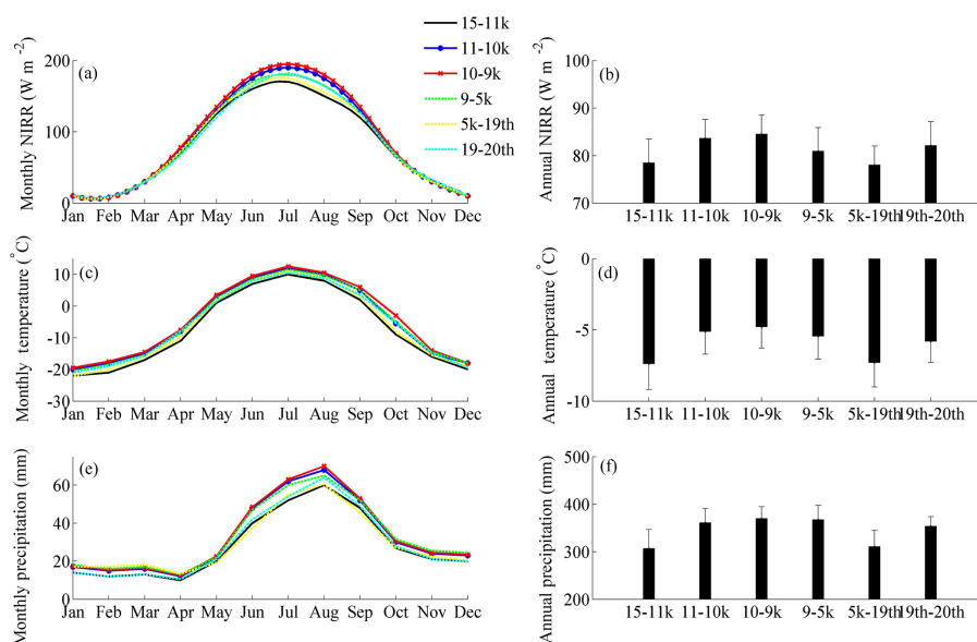
Figure 3. Simulated paleo-climate and other input data from 15 ka to 2000 AD: (a) mean monthly and (b) mean annual net incoming solar radiation (NIRR, \text{W m}^{-2} ), (c) mean monthly and (d) mean annual air temperature ( ^{\circ} ), and (e) mean monthly and (f) mean annual precipitation (mm) (Timm and Timmermann, 2007; He et al., 2014).
