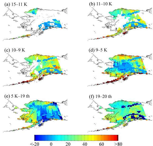
Figure 8. Peatland area expansion and peat soil C accumulation per 1000 years ( \text{kg C m}^{-2} \text{ kyr}^{-1} ) during (a) 15–11 ka, (b) 11–10 ka, (c) 10–9 ka, (d) 9–5 ka, (e) 5 ka–1900 AD, and (f) 1900–2000 AD. The amount of C represents the C accumulation as the difference between the peat C amount in the final year and the first year in each time slice. The period of 9 k–19th in Fig. 2d is separated into 9–5 k and 5 k–19th.
