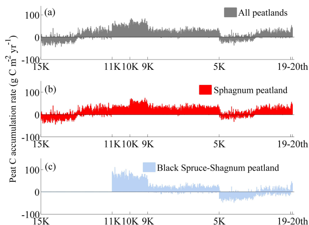
Figure 10. Bars of peatland mean C accumulation rates from 15 ka to 2000 AD for (a) the weighted average of all peatlands, (b) Sphagnum open peatlands, and (c) Sphagnum –black spruce peatlands.
