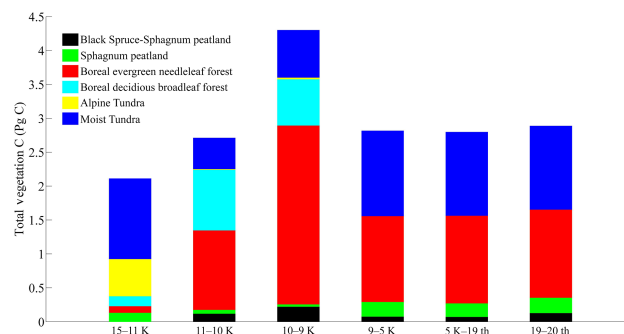
Figure 6. Total C (Pg C) stored in Alaskan vegetation for different time periods.
