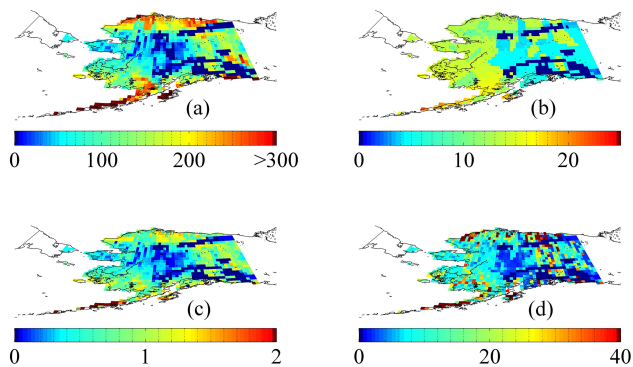
Figure 12. Spatial distribution of (a) total peat SOC density ( \text{kg C m}^{-2} ), (b) total mineral SOC density ( \text{kg C m}^{-2} ), (c) total peat depth (m), and (d) area-weighted total (peatlands plus non-peatlands) SOC density ( \text{kg C m}^{-2} ) in Alaska from 15 ka to 2000 AD.
