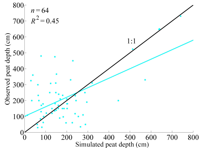
Figure 13. Field-based estimates and model simulations for peat depths in Alaska: the observed and simulated data are extracted from the same grids on the map. The linear regression line (cyan) is compared with the 1 : 1 line. The linear regression is significant ( P < 0.001 , n = 64 ) with R^2 = 0.45 , slope = 0.65, and intercept = 101.05 cm. The observations of > 1000 \text{ cm} are treated as outliers.
