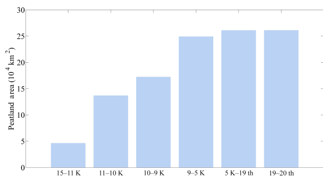
Figure 9. Peatland expansion area ( 10^4 \text{ km}^2 ) in different time slices.
