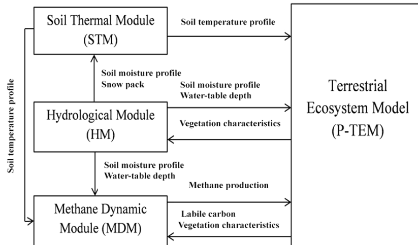
Figure 1. The P-TEM (Peatland-Terrestrial Ecosystem Model) framework includes a soil thermal module (STM), a hydrologic module (HM), a carbon/nitrogen dynamic model (CNDM), and a methane dynamics module (MDM) (Wang et al., 2016).
