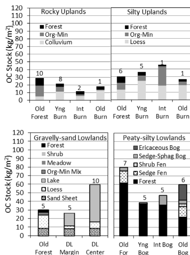
Figure 8. Mean soil organic carbon stocks by soil material for various successional stages (Yng = young, Int = intermediate, DL = drained lake) within four soil landscapes. Totals are for 0–2 m interval, except peaty-silty lowlands, which are for soils of variable depth above a common limnic horizon created after thaw-lake drainage. Patterns represent soil materials of differing origin. Organic materials were differentiated as woody forest or shrub peat, graminoid peat from meadows, fen and bog peat dominated by various lifeforms, and limnic material formed in lakes. Mineral soils were differentiated by geomorphic deposit. Org-Min layers represent turbated mixtures caused by thermokarst. Numbers represent sample sizes.
