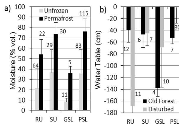
Figure 4. Mean ( \pm SD) soil moisture (a) for unfrozen and frozen soils (all successional stages combined) and water-table depths; (b) for undisturbed old forests and disturbed sites (post-fire) within rocky uplands (RU), silty uplands (SU), gravelly-sandy lowlands (GSL), and peaty-silty lowlands (PSL). Numbers represent sample size for individual samples for moisture and for sites for water table.
