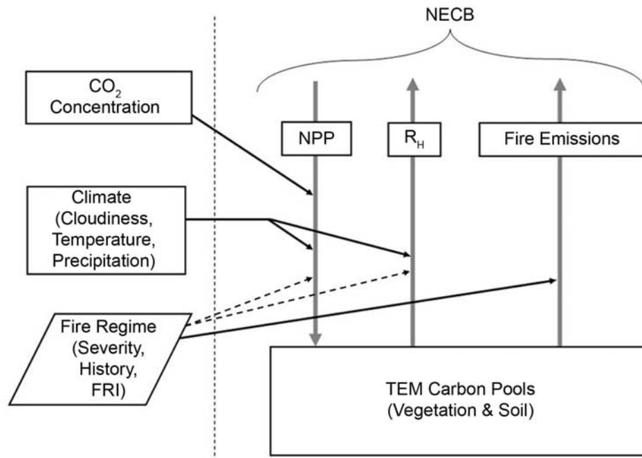
Figure 1. The simulation framework of this study in which the Terrestrial Ecosystem Model (TEM) was used to simulate the effects of fire on carbon dynamics. Input data sets include \text{CO}_2 concentration, cloudiness, air temperature, precipitation, and spatially explicit information on fire history (area burned), burn severity (carbon fraction consumed during a fire event), and fire return interval (FRI, used for inserting fires prior to the historical record). Burn severity parameters, fire history, and FRI are used to calculate fire emissions from TEM carbon pools (vegetation and soil carbon). Fire regime also has indirect effects on net primary production (NPP) and heterotrophic respiration ( R_H ) through the influence on soil and vegetation carbon pools. Model outputs are NPP, R_H , and fire emissions which are used to calculate the net ecosystem carbon balance (NECB).
